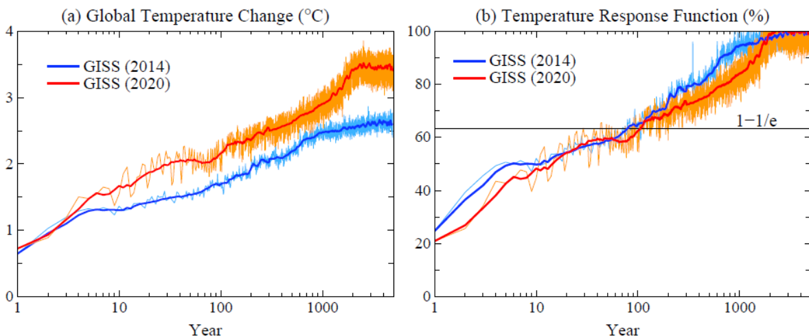
Fig. 3. (a) Global surface temperature response to \text{CO}_2 doubling and (b) normalized response function (% of final change). GISS 2014 and 2020 models have \text{ECS} = 2.7^\circ\text{C} and 3.5^\circ\text{C} .
