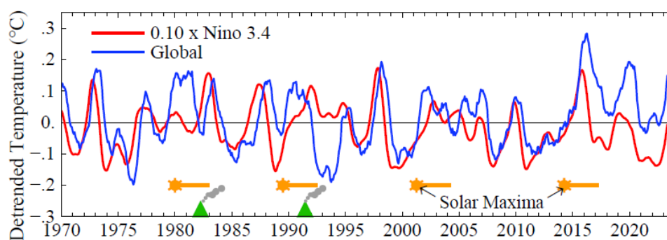
Fig. 5. Detrended global and Nino3.4 12-month running-mean temperatures; the trend subtracted from the temperature records is based on the period 1970-2010.
